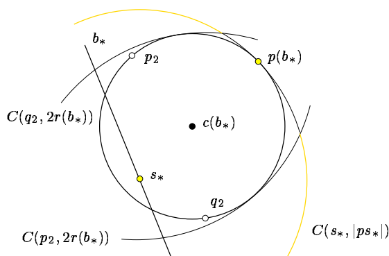
Figure 5: Points satisfying condition (I).
