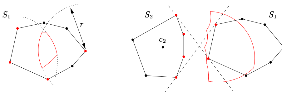
Figure 2: The r_2 -region( S_1 ) (left) and the c_2 -umbrella( S_1, S_2 ) (right).
